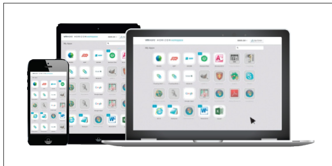
Figure 3. Unified Workspace
